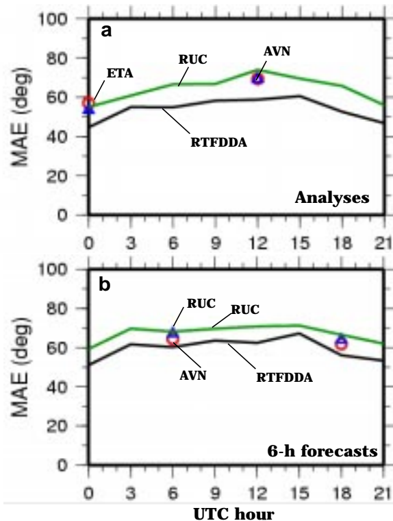
Fig.5 Comparison of wind direction errors of RTFDDA analyses and forecasts with those of RUC, ETA and AVN on the Domain 4, averaged during Feb 3 and April 30
