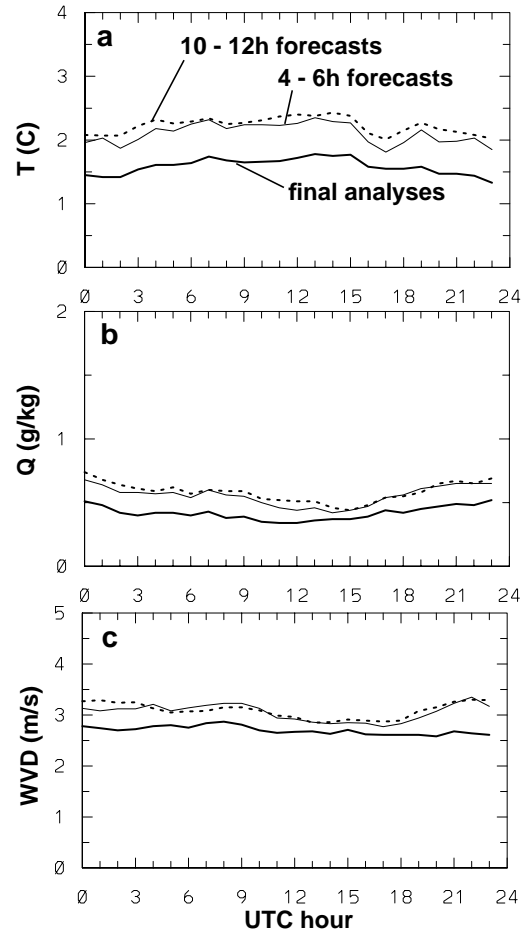
Fig.3 Diurnal changes of the mean absolute errors(MAE) of the rtfd analysis (heavy solid), 4 - 6 hour forecasts (thin) and 10 - 12 hour forecasts (dashed) of the surface temperature (a), specific humidity (b) and wind vector differences (c) on the Domain 4, averaged during the Olympic period (Feb. 6 to Mar. 16, 2002).
