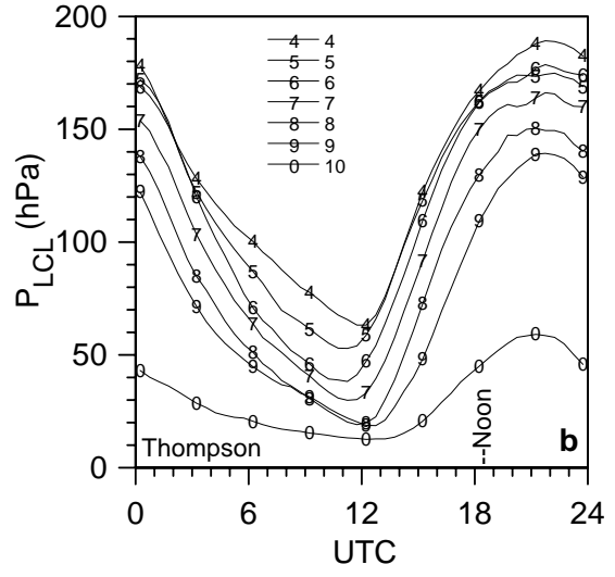
Fig. 8b. As Fig. 8a for P_{LCL} .
