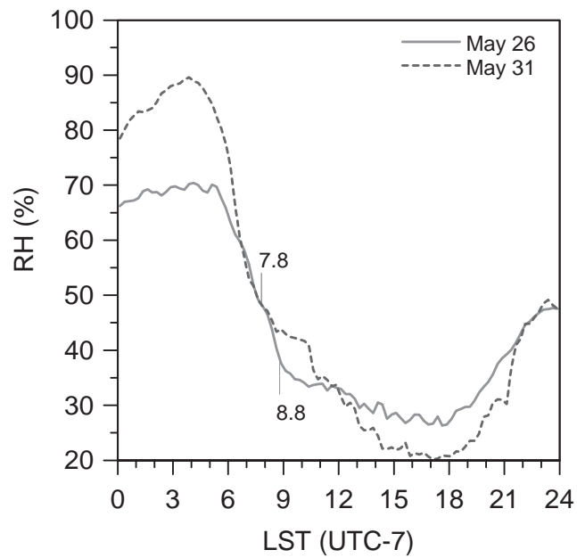
Fig. 2. Diurnal cycle of temperature, above and below a boreal forest canopy (upper panel), and of relative humidity above the canopy (lower panel) for two days in May, 1994.
