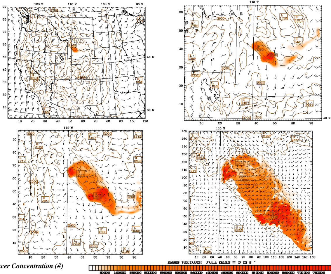
Figure 1. Tracer concentration in the lowest model layer on Domain 1 (upper left), Domain 2 (upper right), Domain 3 (lower left), and Domain 4 (lower right) released from three sources. Wind barbs are in m/s, and terrain in meters. Time is 18 UTC on 7 February 2004.
