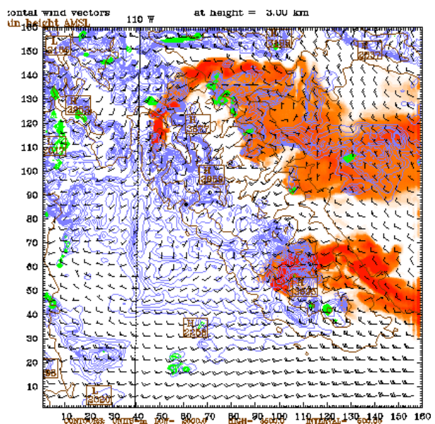
Figure 2. Tracer concentration (orange), cloud water (green contours), and ice (blue contours) at 21 UTC on 7 February 2004. Dark orange greater than 10^4 \text{ kg}^{-1} . Contour intervals for both cloud water and ice are 0.005 \text{ g kg}^{-1} . Maximum contour is 0.2 \text{ g kg}^{-1} .
