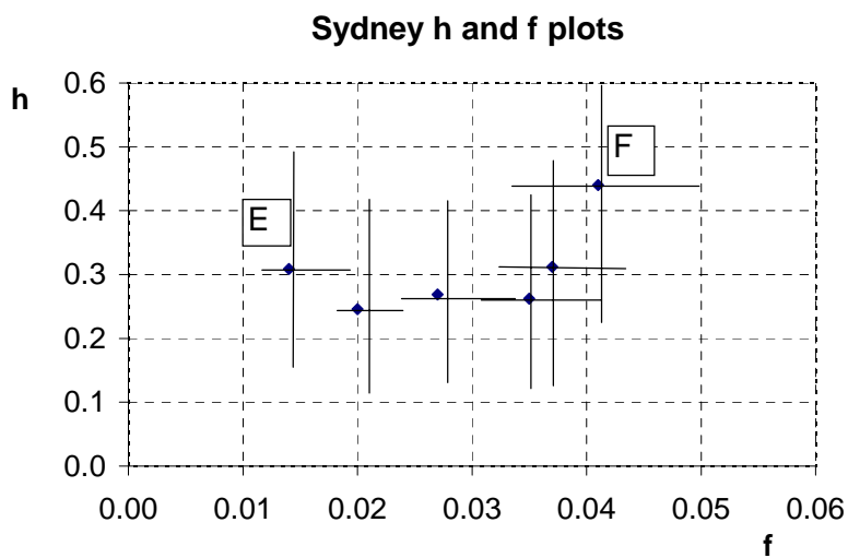
Fig 1. Plots of hit rate vs false alarm rate for individual forecasters at Townsville, Melbourne and Sydney. Error bars are 95% confidence intervals.
